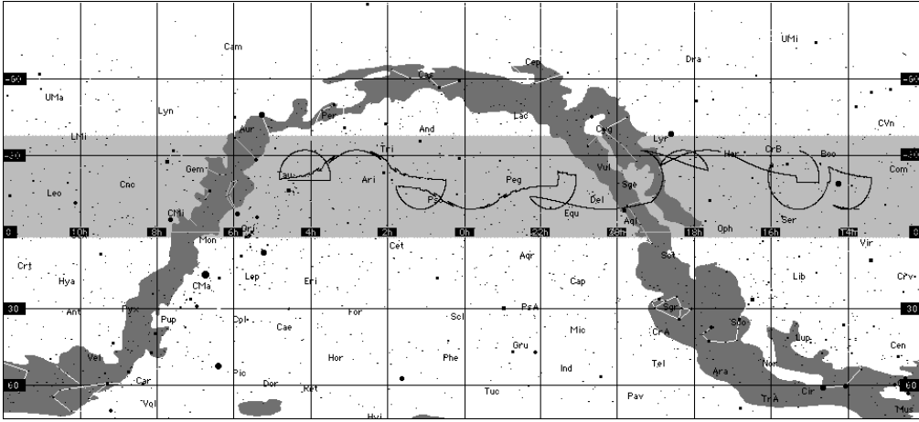
Figure 1. The path of the telescope beam over 15 hours on August 5, 2001.
