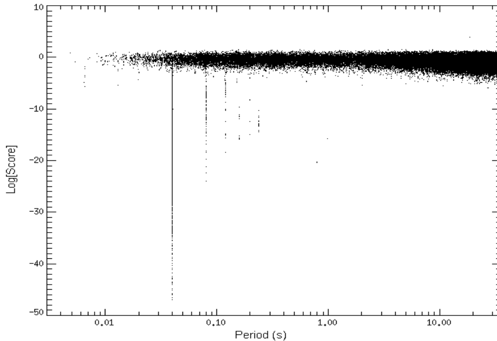
Figure 2. Score distribution vs period for pulse candidates.
