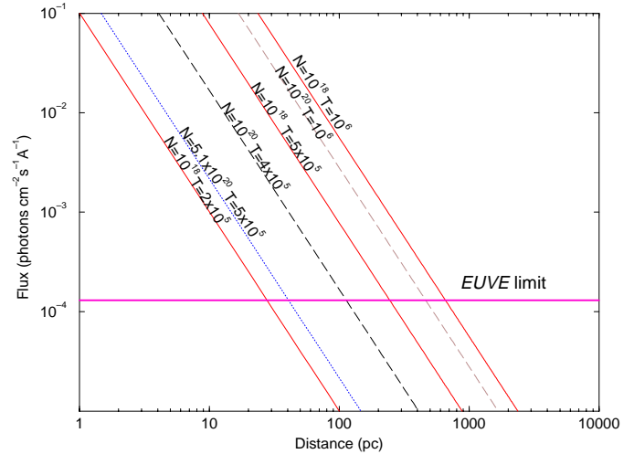
Fig. 1. The obtained EUVE sensitivity ( horizontal thick line ) compared with the fluxes (58–174 Å) for neutron stars as function of distance, temperature and hydrogen column.
